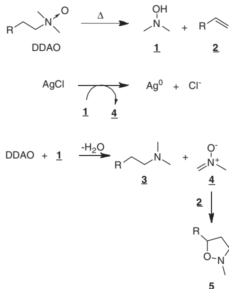
Scheme 1. Proposed chemical reaction in the heating process at 135 °C ( R = C_{10}H_{21} ).
