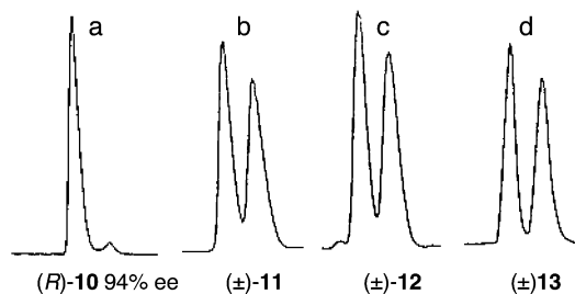
Figure 1. GLC analysis using CHROMPACK Cyclodextrine-b-236M-19 (0.25 × 25 M)
