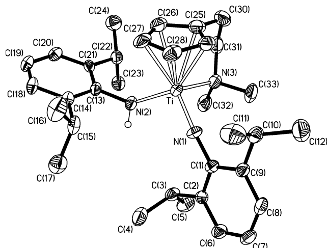
Figure 5. Molecular diagram of \{(2,6\text{-iPr}_2\text{C}_6\text{H}_3)\text{NH}\}\text{Cp}^{\text{N}}\text{-Ti}\{\text{N}(2,6\text{-iPr}_2\text{C}_6\text{H}_3)\} ( 6 ).
