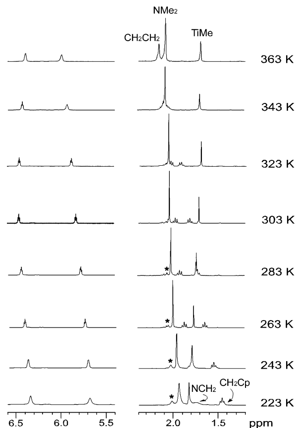
Figure 2. Variable-temperature ^1\text{H} NMR spectra for complex \text{Cp}^{\text{N}}\text{TiMeCl}_2 ( 2 ) (toluene- d_8 ). *Denotes residual solvent peak.
