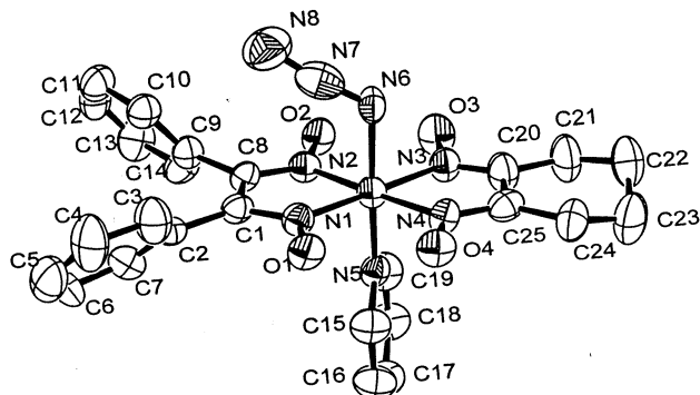
Fig. 3. ORTEP plot of structure \text{N}_3\text{Co}(\text{chgH})(\text{dpgH})\text{Py} ( 8b ).
