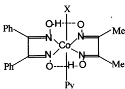
Fig. 1. Structure of cobaloximes.
