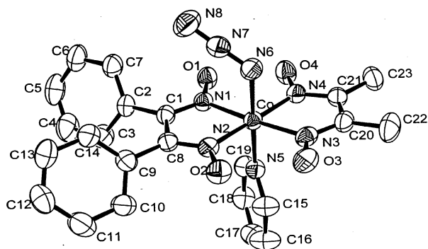
Fig. 2. ORTEP plot of structure \text{N}_3\text{Co}(\text{dmgH})(\text{dpgH})\text{Py} ( 4b ).
