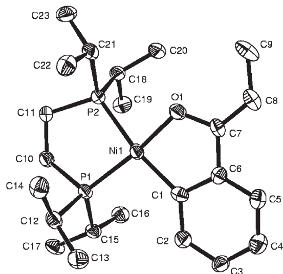
Figure 1. View of the molecular structure of complex 8b together with the atomic numbering system. Selected bond lengths [Å] and angles [°]: Ni–O1 1.853(3) , Ni–Cl1 1.913(4) , Ni–P1 2.1627(12) , Ni–P2 2.2064(12) , O1–C7 1.342(5) , C7–C8 1.368(6) , C6–C7 1.464(6) , C1–C6 1.398(6) , C8–C9 1.496(7) ; O1–Ni–Cl1 86.17(15) , C1–Ni–P1 99.77(12) , O1–Ni–P2 86.10(10) , O1–C7–C8 119.7(4) , Ni–O1–C7 115.4(2) , O1–C7–C6 113.0(3) , C6–C7–C8 127.3(4) , C7–C8–C9 122.6(5) , P1–Ni–P2 88.50(5) .
