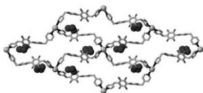
Figure 5. Top view of the 2D sheet structure of 7 . Hydrogen atoms and nitrate anions have been omitted for clarity. The guest molecules are represented by a space filling model. One of the guest molecules is disordered.
