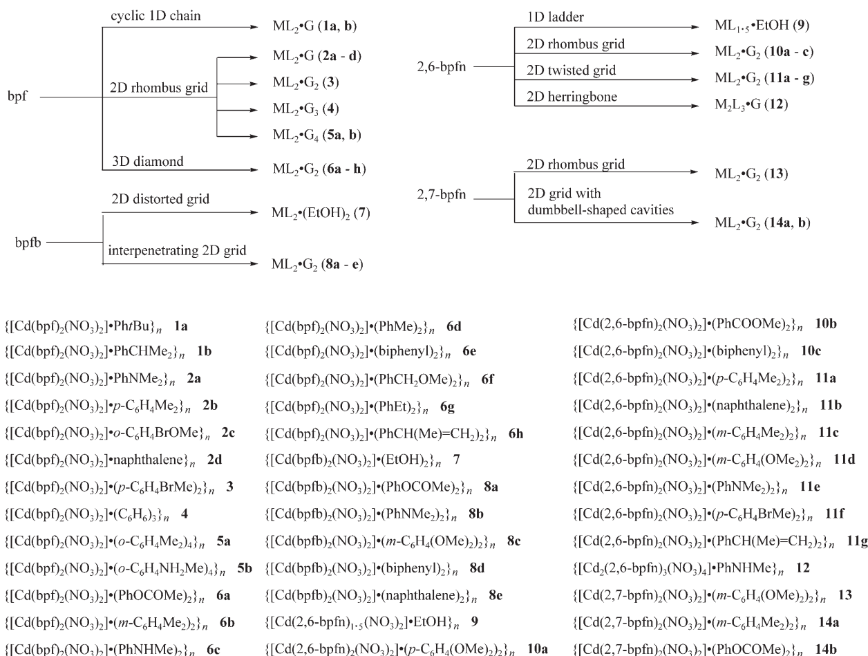
Scheme 2. Preparation of 1a , 2a–d , 3 , 4 , 5a , 5b , 6a–h , 7 , 8a–e , 9 , 10a–c , 11a–g , 12 , 13 , 14a , and 14b .
