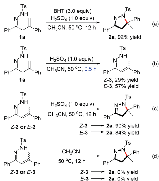
Scheme 3 Control experiments.
