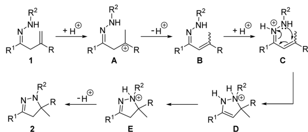
Scheme 4 Proposed mechanism.
