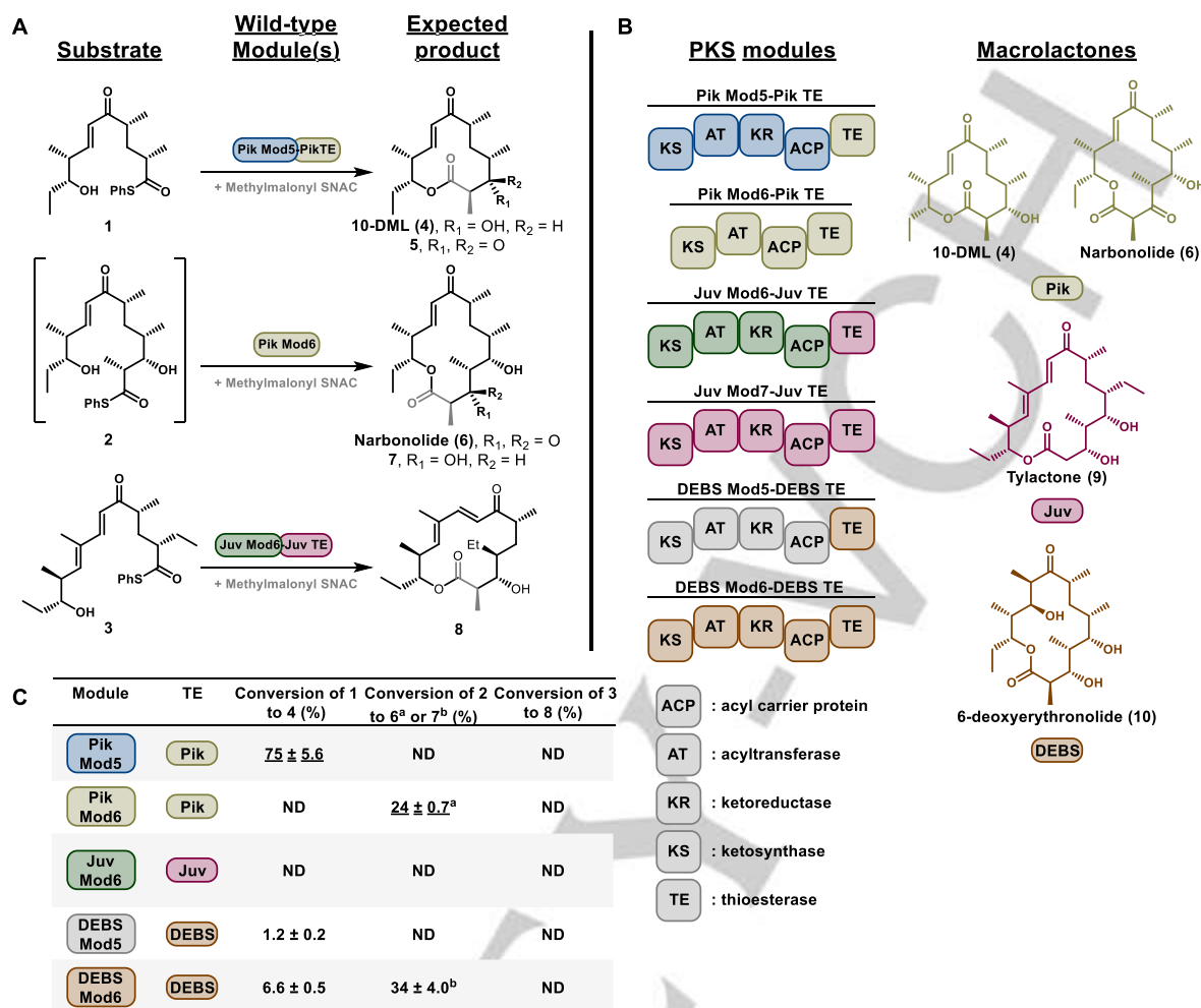
Figure 1. (a) Reaction scheme of PKS modules processing their native full-length synthetic substrates 1 4a , 2 4b , 3 4c to the corresponding macrolactones. Substrate 2 is generated by in situ photolysis of the 2-nitrobenzyloxymethyl ether (NBOM) protected native hexaketide. 4b (b) Domain architecture of the PKS modules used in this study and the native macrolactone products from each respective biosynthetic pathway. (c) Table of percent conversion for reactions with substrates 1-3 . The product yield for each PKS module processing its native substrate is underlined. Conversion to each macrolactone was monitored by HPLC with data represented as the mean ± standard deviation where n = 3. ND = not detected.
