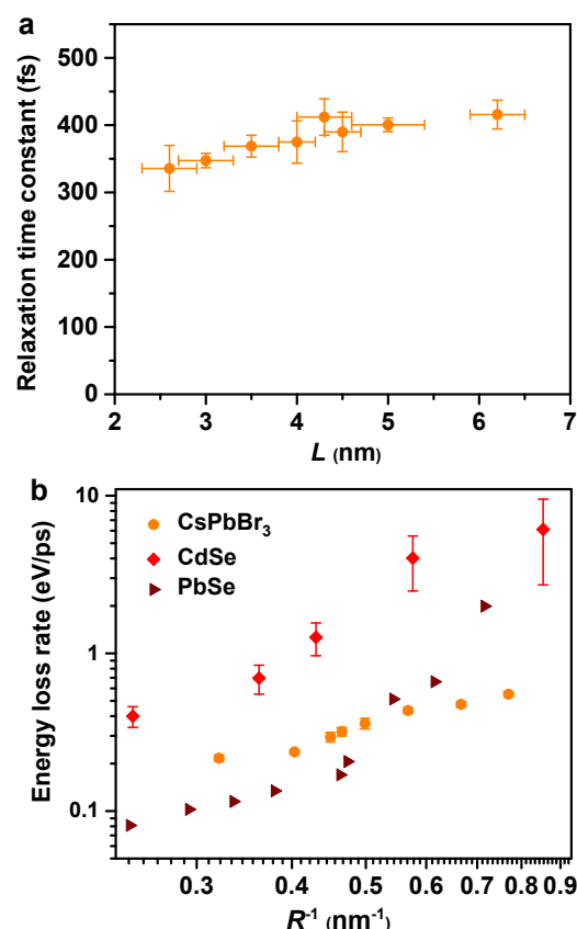
Figure 2. Hot exciton relaxation time constants (a) and hot carrier energy loss rates (b) of CsPbBr 3 NCs as a function of NC size (orange circles). Note that in order to compare cube-like CsPbBr 3 NCs with previous reports on spherical QDs in (b), we define R = L/2 for these
