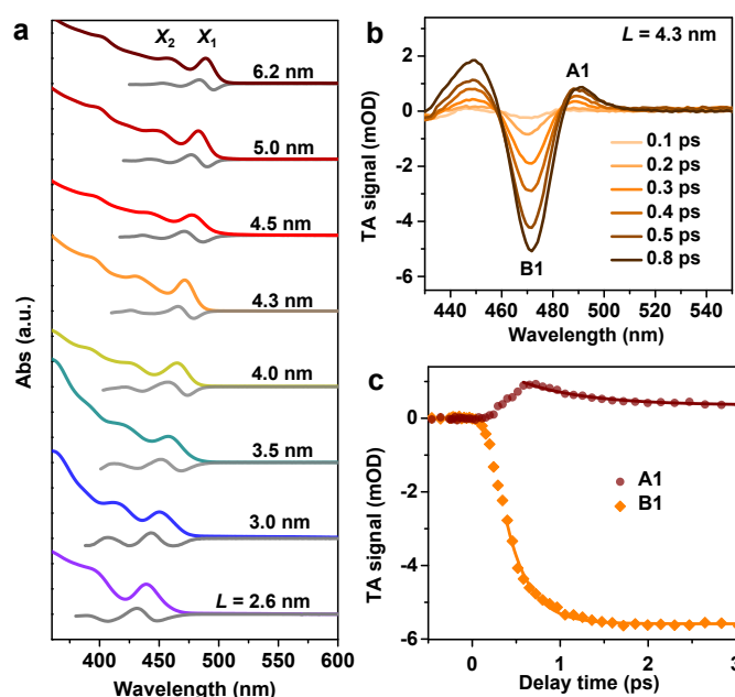
Figure 1. (a) Absorption (colored lines) and first derivative of absorption (gray lines) spectra of NCs of varying sizes. The positions of X_1 and X_2 on these spectra are labelled. (b) Transient absorption (TA) spectra of L = 4.3 nm NCs at indicated delays following the excitation by a 430 nm pulse. The bleach feature B1 and absorptive feature A1 are labelled. (c) TA Kinetics probed at the peaks of A1 (wine circles) and B1 (orange diamonds) are their single-exponential fits (solid lines).
