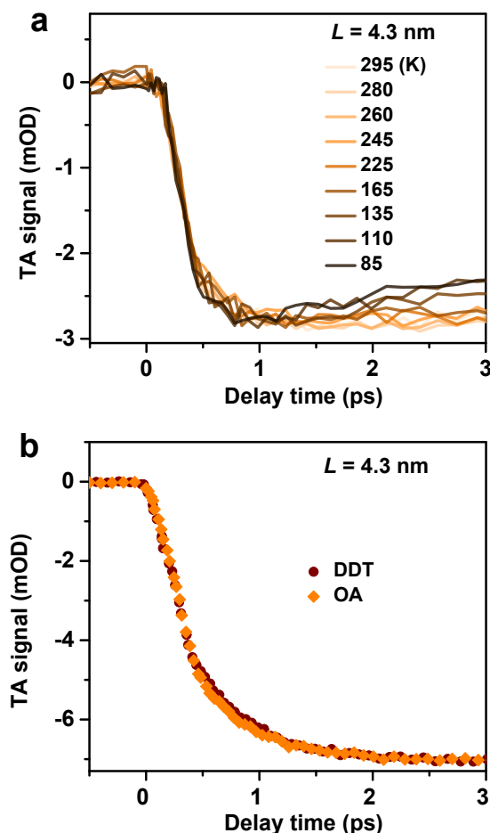
Figure 3. (a) Hot exciton relaxation dynamics (monitored at B1) for L = 4.3 nm NCs at varying temperatures. (b) Hot exciton relaxation dynamics (monitored at B1) for L = 4.3 nm pristine NCs (with OA ligands; orange diamonds) and DDT-capped NCs (wine circles).
