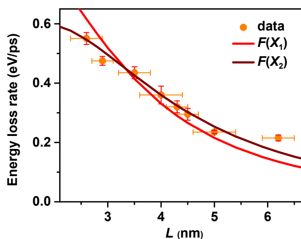
Figure 4. Measured hot carrier energy loss rates (orange circles) and calculated wavefunction surface fraction ( F ) of X_1 (red solid line) and X_2 (wine solid line) for CsPbBr 3 NCs of varying sizes. F(X_1) and F(X_2) have been appropriately scaled by constant factors.
