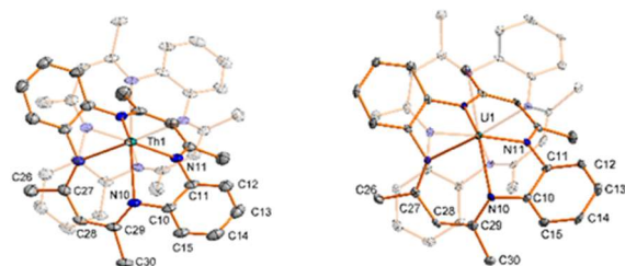
Figure 1. Molecular structure of 1 (left) and 2 (right). The “apical ligand” of the sandwich complexes are faded out for clarity. Hydrogen atoms, as well as additional solvents, have been omitted for clarity. Ellipsoids are shown at a probability level of 50 %.
