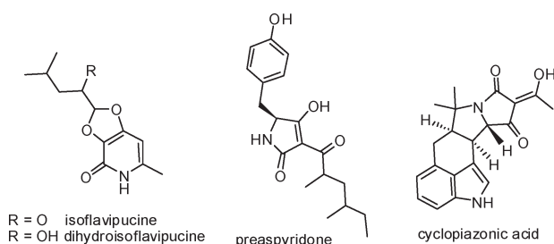
Figure 1. Selected tetramic acid natural products.
