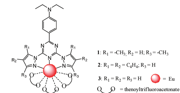
Figure 1. The molecular structures of europium complexes (1–3) with triazine-based ligands.
