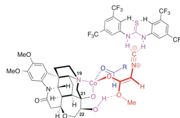
Figure 1. Proposed stereomodel for cooperative catalysis.
