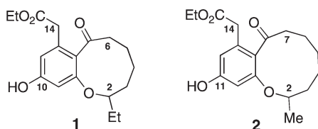
Figure 1. Structures of phomopsins A ( 1 ) and B ( 2 ).
