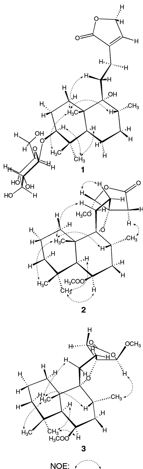
Fig. 3. Key NOE Correlations Observed for 1 , 2 , and 3
