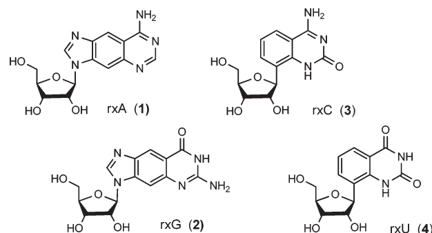
Figure 1. The xRNA genetic set.
