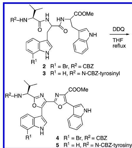
Scheme 2. Moody Biomimetic Oxazole Formation
