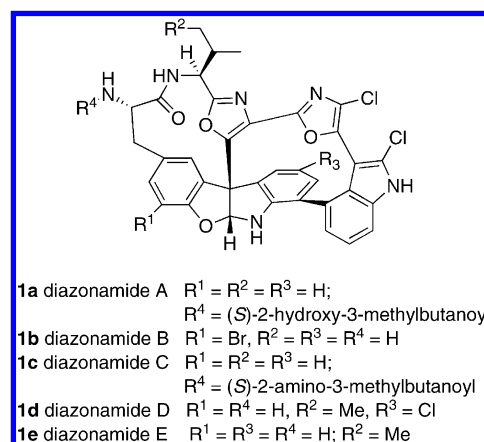
Scheme 1. Structures of Diazonamides A–E
