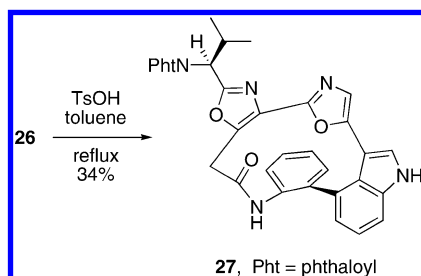
Scheme 7. Robinson–Gabriel Route to Macrocyclic Bis-oxazole 27
