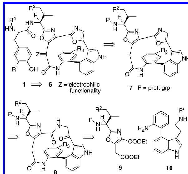
Scheme 3. Approach to Diazonamides
