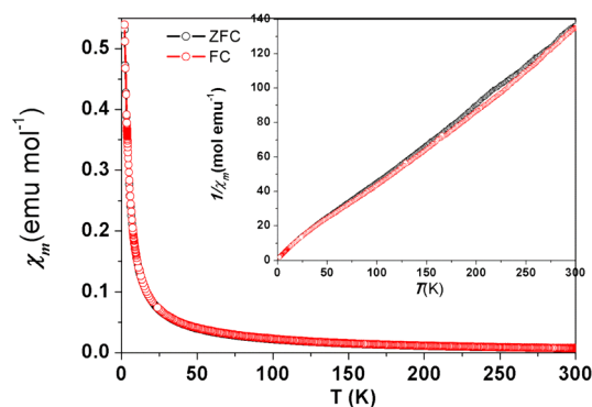
Figure 3. \chi_m versus temperature of Ba 2 NdGaS 5 for FC and ZFC data. Inset: plot of 1/\chi_m versus temperature.
