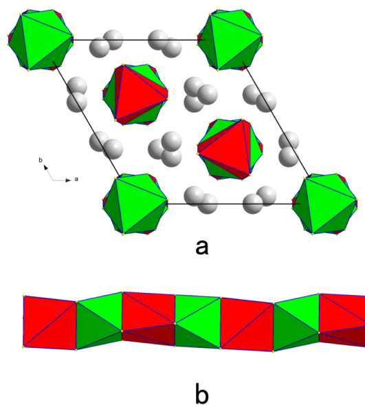
Figure 1. Crystal structure (a) and the [\text{GdInS}_6]^{6-} anionic chain (b) of \text{Ba}_3\text{GdInS}_6 (GdS 6 and InS 6 polyhedra are shaded in red and green, respectively; the white balls are Ba atoms).
