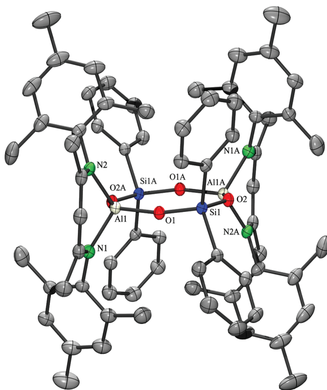
Figure 1. Molecular structure of 3. Hydrogen atoms and solvent molecules are omitted for clarity. Thermal ellipsoids are set at 50% probability. Selected bond lengths (Å) and angles (deg): Al1–O1 1.707(2), O1–Si1 1.600(2), Si1–O2 1.615(2), O2–Al1A 1.714(2); Al1–O1–Si1 137.4(1), O1–Si1–O2 112.8(1), O2–Al1A–O1A 115.7(1).
