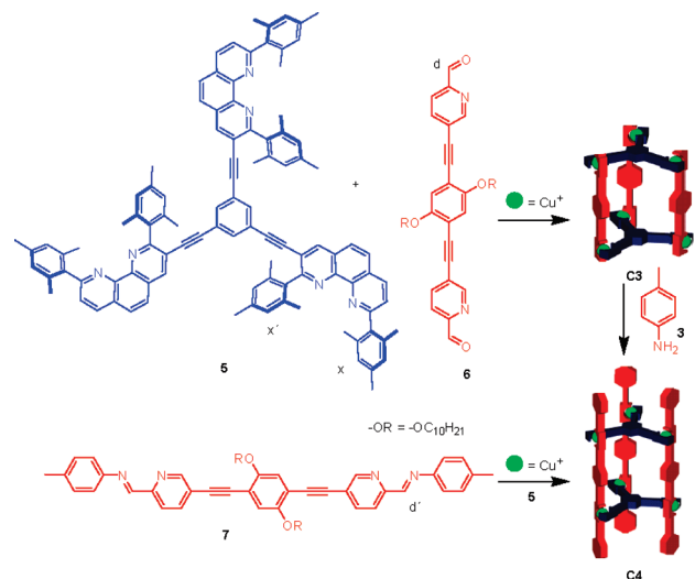
Scheme 3. Synthesis of Nanoprism C3 and C4
