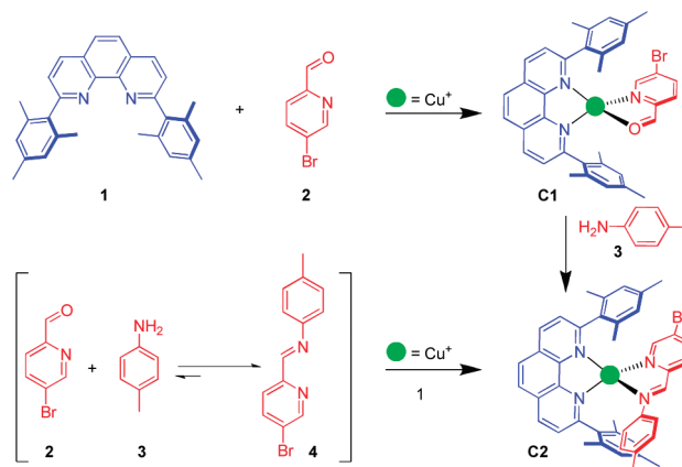
Scheme 2. Synthesis of Heteroleptic Complexes C1 and C2
