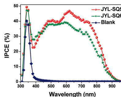
Figure 3. Incident monochromatic photon-to-current conversion efficiency (IPCE) spectra of the devices sensitized by JYL-SQ5 or JYL-SQ6 and a blank device (without dye).
