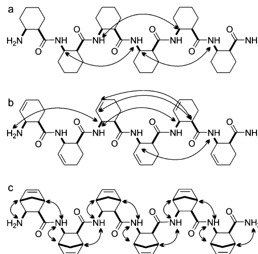
Figure 2. Long-range NOE interactions for (a) 2 in \text{CDCl}_3 and for (b) 4 and (c) 6 found in DMSO and \text{CD}_3\text{OH} .
