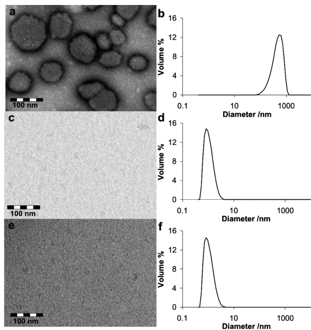
Figure 4. TEM images of (a) 2 , (c) 4 , and (e) 6 and DLS curves for (b) 2 , (d) 4 , and (f) 6 as 4 mM solutions in water.
