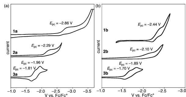
Figure 4. Cyclic voltammograms of (a) 1a – 3a and (b) 1b – 3b in THF, measured with [n\text{-Bu}_4\text{N}][\text{PF}_6] (0.1 M) as a supporting electrolyte at a scan rate of 100 \text{ mV s}^{-1} .
