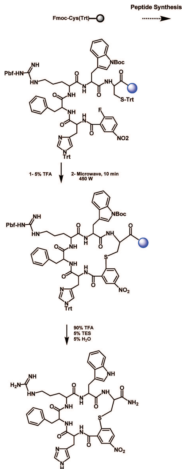
Scheme 1. General Synthetic Method for Macroyclic Melanocortins
