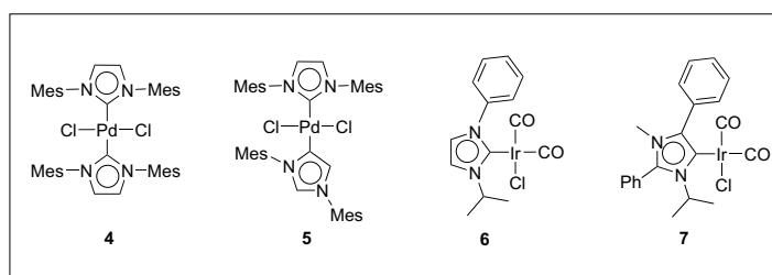
Fig. 1. Normal and abnormal NHC complexes of palladium(II) and iridium(I)
