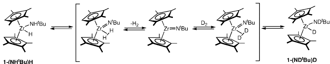
Figure 9. Proposed mechanism for intra- and intermolecular isotopic exchange with the amide hydrogen and the zirconium hydride.
