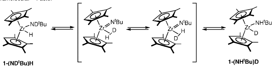
Figure 8. Free energy profiles for evaluating 1,2-elimination (top) versus reductive coupling (bottom) for intramolecular isotopic exchange for (\eta^5\text{-C}_5\text{H}_5)_2\text{Zr}(\text{NH}^t\text{Bu})\text{H} . A = (\eta^5\text{-C}_5\text{H}_5)_2\text{Zr}(\text{NH}^t\text{Bu})\text{H} , B = (\eta^5\text{-C}_5\text{H}_5)_2\text{Zr}(\text{N}^t\text{Bu})(\eta\text{H}_2) , C = (\eta^5\text{-C}_5\text{H}_5)_2\text{ZrNH}_2^t\text{Bu} .
