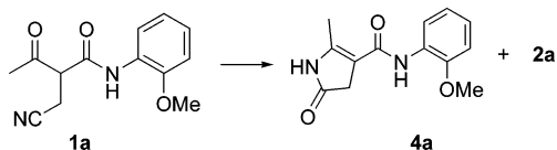
SCHEME 5. Reaction of 1a in the Presence of 0.2 or 0.5 equiv of SnCl 4 ·5H 2 O
