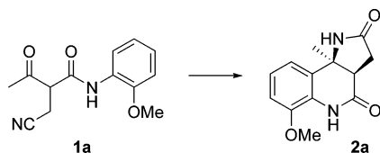
SCHEME 2. Synthesis of Pyrrolo[3,2- c ]quinoline 2a from 1a
