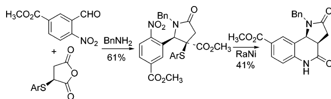
SCHEME 2. Synthesis of Pyrrolo[3,2- c ]quinoline 2a from 1a
