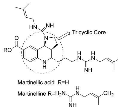
FIGURE 1. Structures of martinellac acid and martinelline.
