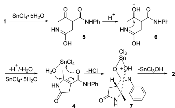
SCHEME 5. Reaction of 1a in the Presence of 0.2 or 0.5 equiv of SnCl 4 ·5H 2 O
