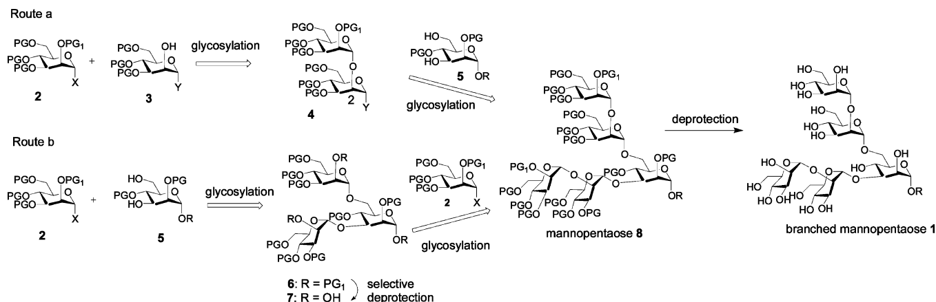
FIGURE 1. Two general approaches for the synthesis of branched mannopentaoses.
