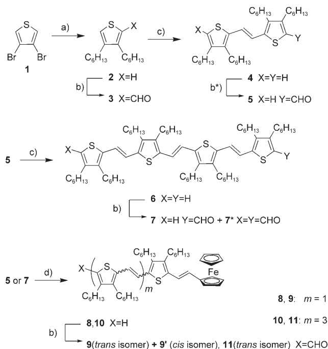
Scheme 1. Synthesis of n TVs: a) C_6H_{13}MgBr , [NiCl_2(dppp)] , dry THF, reflux; b) POCl_3 , dry DMF/DCE, reflux; b*) 1) POCl_3 , dry DMF/DCE, reflux; 2) I_2 , dry toluene, reflux; c) TiCl_4 , Zn/dry THF, reflux; d) TiCl_4 , Zn/dry THF, ferrocenecarboxaldehyde, reflux.
