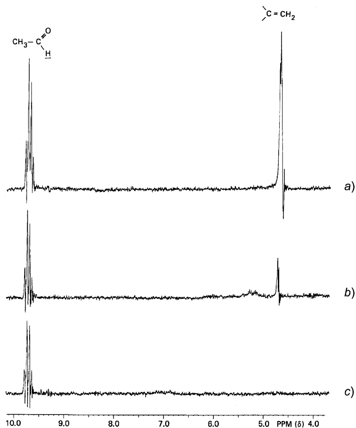
Fig. 1. CIDNP Spectra during the photolysis of a) DMB, b) EMP, and c) PMIK in \text{CD}_3\text{CN} solution
