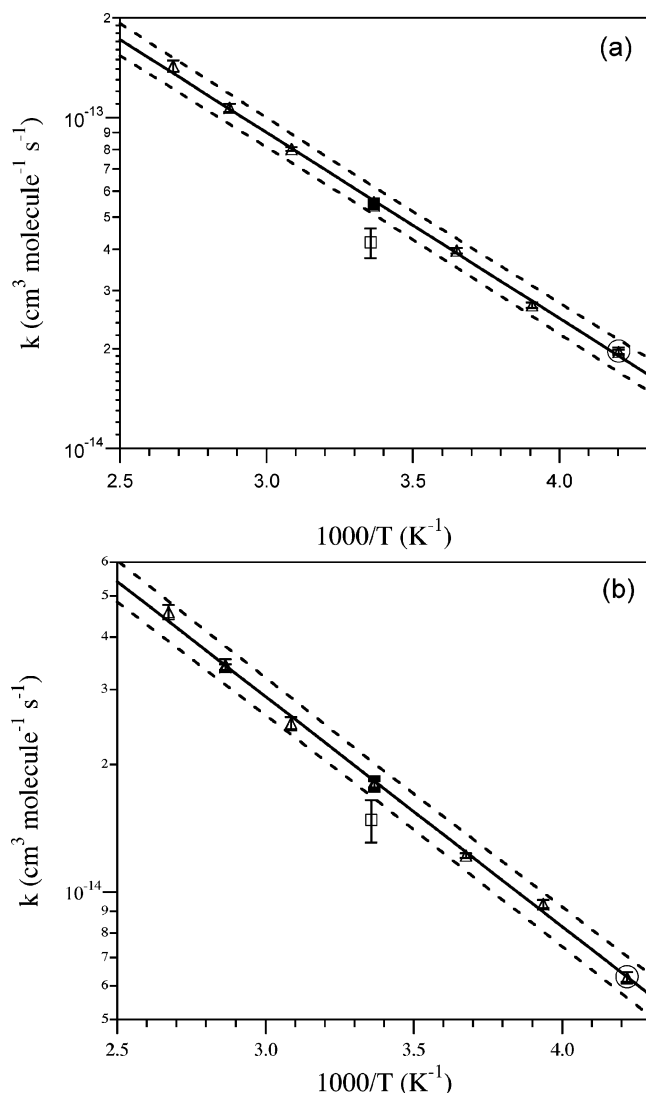
Figure 2. Arrhenius plot for the rate coefficient data obtained for the OH radical reaction with (a) \text{CF}_3\text{CH}_2\text{CH}_3 ( k_1 ) and (b) \text{CF}_3\text{CHFCH}_2\text{F} ( k_2 ) over the temperature range 238–373 K. The triangles correspond to data obtained with the unpurified sample and the circles to the data obtained with a purified sample. The solid lines are the linear least-squares fit to all the data (see text for details). The dashed lines represent the 2\sigma uncertainty limits, f(T) , calculated using f(298 \text{ K}) = 1.10 and g = 20 (see text for definition of terms). The open squares are the room-temperature values reported by Nelson et al. 3
