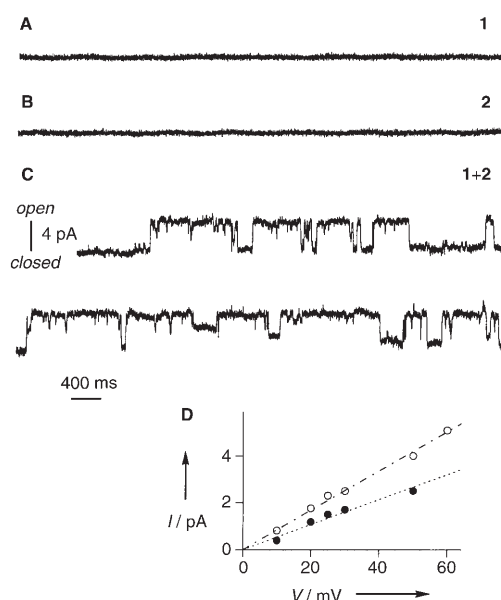
Figure 2. Planar EYPC bilayer conductance in the presence of A) 1 ( 5\ \mu\text{M} cis ), B) 2 ( 2.4\ \mu\text{M} cis ) and C) 1 ( 5\ \mu\text{M} cis ) and 2 ( 2.4\ \mu\text{M} cis ) at +50\ \text{mV} ( trans at ground) in 2\ \text{M} KCl. D) IV profile of two different frequent single-channel current levels (open and closed circles) with linear curve fit.
