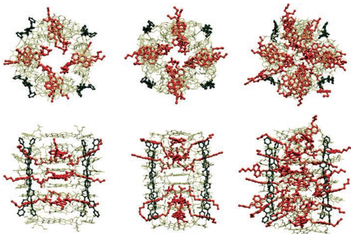
Figure 3. Optimized geometry of molecular models of complexes 1 4 .2 12 (left, barrel length l=38 Å, inner diameter d=5.4 Å), 1 4 .2 16 (middle, l=42 Å, d=3.0 Å) and 1 4 .2 28 (right, l=45 Å, d=2.0 Å) in side (bottom) and axial view (top). p -Octiphenyl staves (dark green) and DAN ligands (red) are both in ball-and-stick representation, NDI hoops (light green) are in wire representation, H omitted, 50% (left) to 100% (middle, right) amine protonation, 0% sulfate protonation ( 1 4 .2 12 is adapted from [36] with permission, Copyright 2005 Am. Chem. Soc.).
