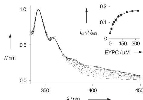
Figure 4. Emission spectra of 2 (20 \mu\text{M} ) with increasing concentration of EYPC LUVs [0 (----) \rightarrow 330 \mu\text{M} EYPC (—), \lambda_{\text{ex}} 325 nm]. Inset: Fractional emission intensity I_{410}/I_{343} as a function of lipid concentration with curve fit to the White equation. [41]
