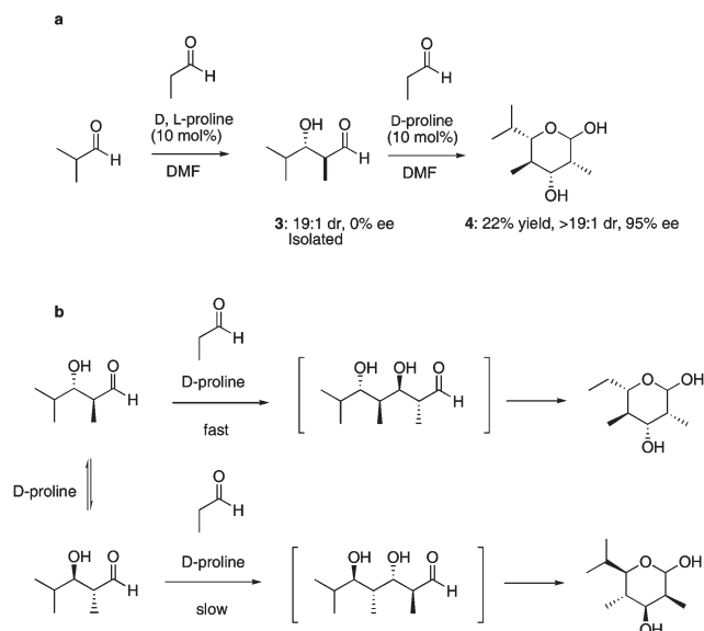
Scheme 1 (a) A two-step synthesis of a polyketide hexose. The first step is performed with racemic proline and the next step with enantiomerically pure D-proline. (b) The potential mechanism of the D-proline catalyzed anti -selective aldol reaction step.
