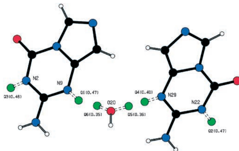
Fig. 6. Residual electron-density peaks (green) in the final refinement stages demonstrate the co-existence of two tautomeric forms (numbers in parentheses in electrons per \text{\AA}^3 ). In this crystal structure, a fully occupied H-atom can be expected to appear with a peak height of ca. 0.8 \text{ e}^-/\text{\AA}^3 in the DF map.
