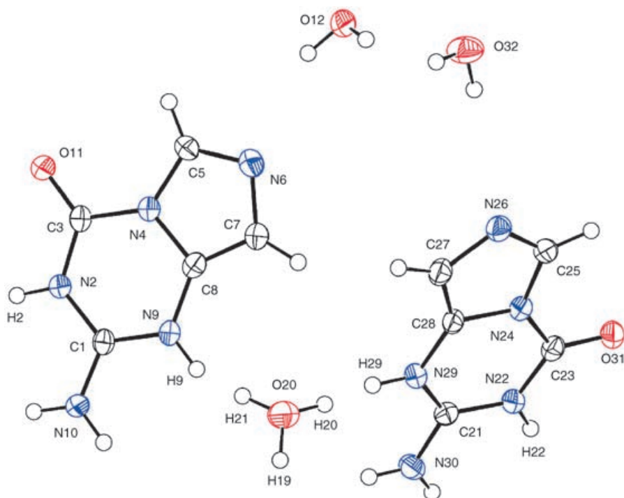
Fig. 4. Structure of compound 4 in the crystal [13]. The asymmetric unit comprises two independent molecules (I and II) of alloG and three molecules of H 2 O. Atomic displacement ellipsoids drawn at the 50% probability level, H-atoms drawn as spheres of arbitrary radius. The H-atoms H(2)/H(22), H(20)/H(21), and H(9)/H(29) are disordered over two sites with a 0.5:0.5 distribution.
