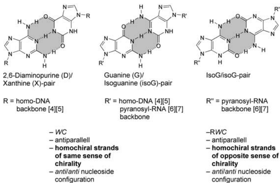
Fig. 2. Watson–Crick (WC) and reverse-Watson–Crick (RWC) modes of purine–purine base-pairing observed in the homo-DNA and pyranosyl-RNA series
