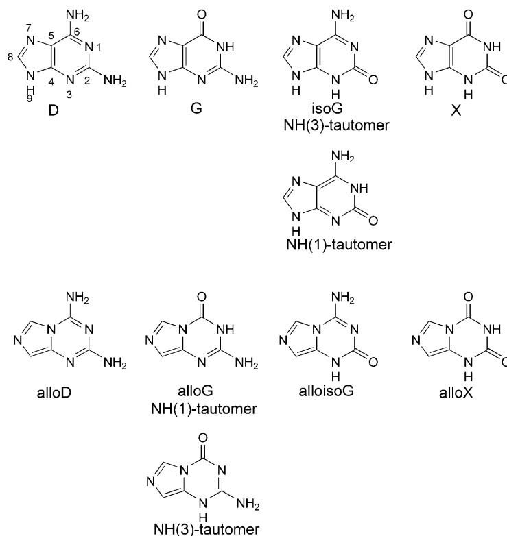
Fig. 1. Juxtaposition of the chemical formulae of members of the purine family with those of corresponding member of the 'allo-purine' family
