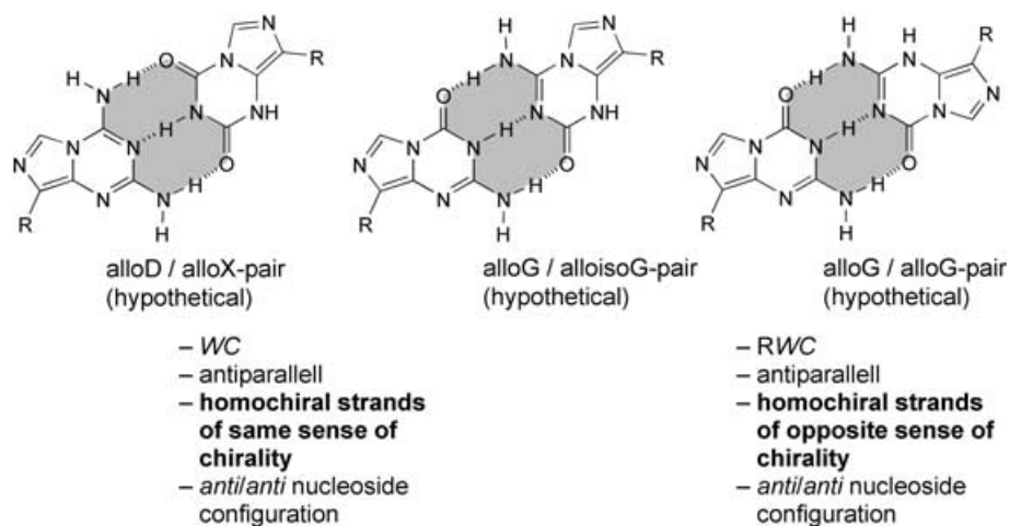
Fig. 3. Watson–Crick (WC) and reverse-Watson–Crick (RWC) modes of (hypothetical) allopurine–allopurine base-pairing in informational oligomers
