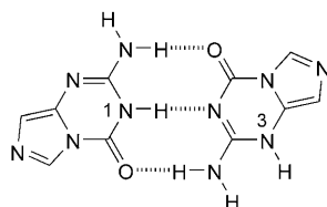
Fig. 7. Triply H-bonded motif observed for both independent molecules of alloG in the crystal. One half of the molecules are present in the NH(1) tautomeric form and the other half in the NH(3) form (allopurine numbering).
