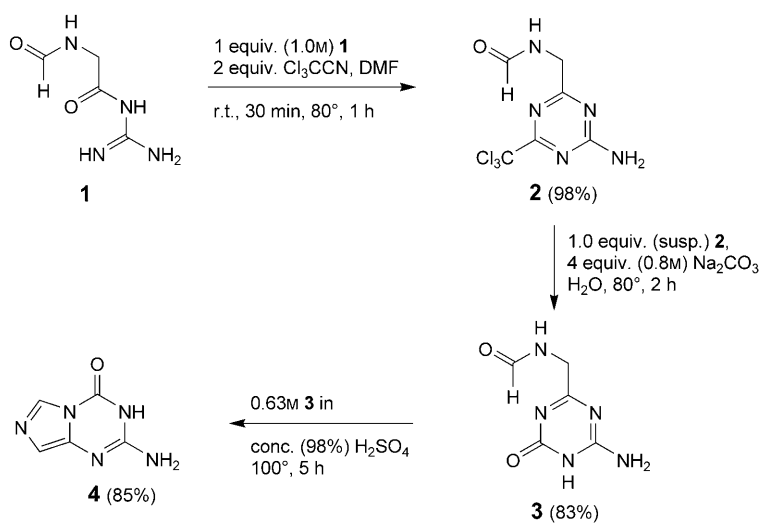
Scheme. Synthesis of 5,8-Diaza-7,9-dicarbapurine ('Alloguanine'; 4 )
