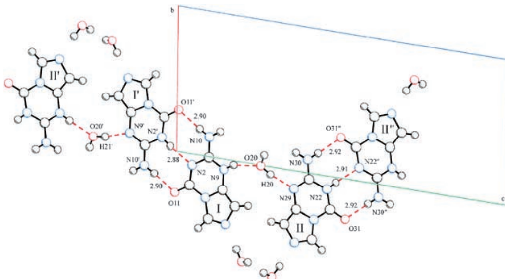
Fig. 5. Packing of alloG in the crystal (view down a ) visualizing the co-existence of the two tautomers and the reverse-Watson–Crick pairing of molecules I and II with their symmetry mates [14]. Primed/double-primed atoms are related to unprimed atoms by the crystallographic symmetry operations 1 - x, -y, -z (inversion center between N(2) and N(2')) and 1 - x, -y, 1 - z (inversion center between N(22) and N(22')); molecules I and I' ( II and II' ) are coplanar. The H-atoms at N(2') and N(22) are disordered about the centers of symmetry. H-Bond donor/acceptor distances in Å. For each disordered site only one orientation is shown.
