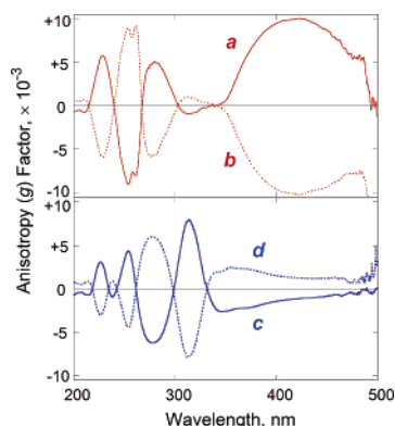
Figure 3. Electronic circular dichroisms of enantiopure 1 (a and b) and 2 (c and d) in acetonitrile. Only anisotropy ( g ) factors are shown for clarity (see Supporting Information for full UV–vis and ECD spectra). Solid lines are for the (–)-enantiomer.
