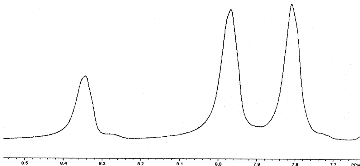
Fig. 2. Bound phenyl region of the ^1\text{H} -NMR spectrum of 2 in \text{CDCl}_2\text{F} – \text{CDClF}_2 at -135\text{ }^\circ\text{C} .
