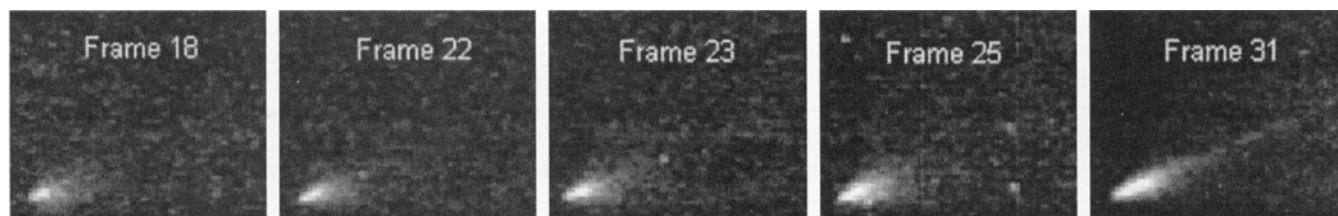
FIG. 3. Typical diffuse structures for the LN98023 fireball recorded by the LLTV system. Field of view of each frame is 6.0 \times 4.8^\circ . Altitudes and distances for individual frames are given in Table 3.
