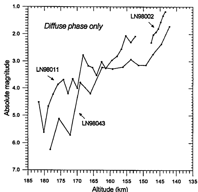
FIG. 9. Lightcurves of the LN98002, LN98011, and LN98043 fireballs.
