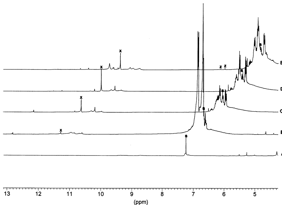
Fig. 3. Partial ^1\text{H} -NMR spectra of reaction mixture containing 3 and \text{PhC}\equiv\text{CH} in \text{CDCl}_3 at 293 K, demonstrating the coordination of \text{PhC}\equiv\text{CH} to tungsten ( \delta 11.90 ppm) and formation of 1,3,5-TPB and 1,2,4-TPB ( \delta 7–8 ppm). (A) Before addition of \text{PhC}\equiv\text{CH} ; (B), (C), (D) and (E) after 10 min, 6 h, 24 h, and 96 h reaction, respectively. The signals are denoted as follows: (s) proton impurities in the solvent; (x) hydrogens of -\text{CH} groups in [\text{WCl}_2(\text{CO})(\text{NCMe})(\text{PhC}\equiv\text{CH})_2] 13 ( \delta 11.90 ppm); (z) hydrogens in tungstenacyclopentadiene ( \delta 8.53, 8.67 ppm).
