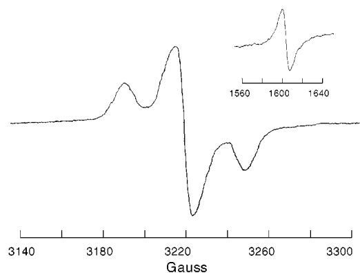
Figure 4. ESR spectrum of \mathbf{3}^{2+} in PrCN at 100 K.
