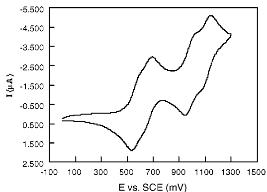
Figure 2. Voltammogram of 3 (1.0 mM) at 298 K in \text{CH}_2\text{Cl}_2 (0.1 M \text{Bu}_4\text{NBF}_4 ) with scan rate of 20 \text{ mV s}^{-1} .
