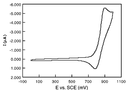
Figure 3. Voltammogram of 4 (1.0 mM) at 298 K in \text{CH}_2\text{Cl}_2 (0.1 M \text{Bu}_4\text{NBF}_4 ) with scan rate of 20 \text{ mV s}^{-1} .
