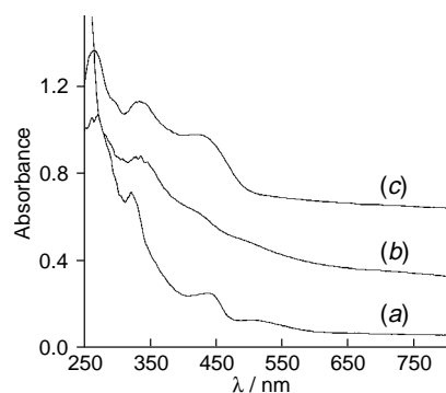
Fig. 2 UV-VIS spectra (in diffuse reflectance mode) of oxidized 1 in solution (a), 1 -EMT (b) and 3 -EMT containing \text{Mn}^{\text{II}} complexed by the salen ligand of 1 (c)
