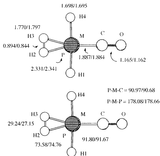
Figure 2. Optimized transition states for hydride exchange in \text{MH}_4(\text{CO})(\text{PH}_3)_2 . Distances are in Å, top drawing; angles are in degrees, bottom drawing. All distances are from M to indicated atom, unless otherwise noted. The first value in any pair is for Os, the second for Ru.
