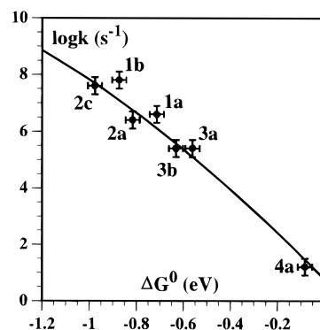
Figure 1. Variation of the cleavage rate constant with the standard free energy of the reaction.
