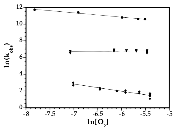
Figure 8. Reaction order plot showing the effect of [O_2] (0.2–4.4 mM) on the observed second-order rate constant for the decay of peroxide intermediates 1b (5 °C, diamonds), 2b (22 °C, circles), and 3b (55 °C, triangles); 0.15–0.75 mM.
