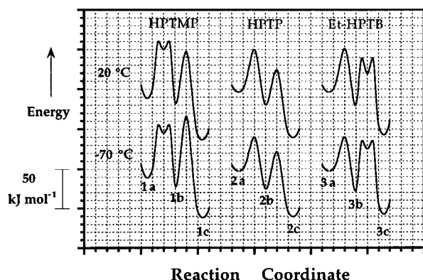
Figure 10. Reaction coordinate diagram showing \Delta G^\ddagger for the reactions of 1a – 3a with dioxygen at +20 and –70 °C.
