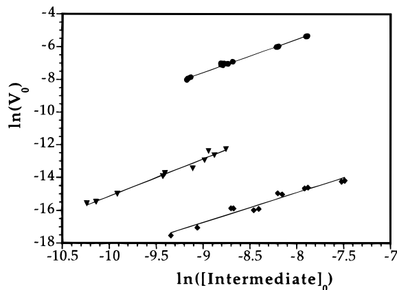
Figure 7. Reaction order plot showing the \ln(V_0) for peroxide intermediate decomposition versus \ln([1b, 2b, 3b]) , the concentration at which second-order decomposition is observed to begin: 1b , diamonds; 2b , circles; 3b , triangles.
