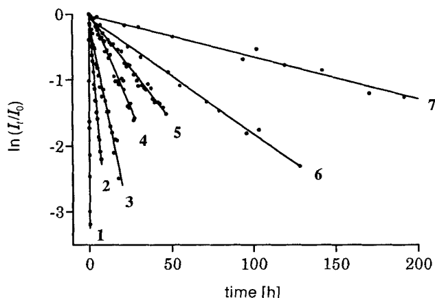
Fig. 2. Pseudo-first-order rate plots for the deuteration of the investigated 5-monosubstituted hydantoin 1–7 at 50°C. I_t : integral of exchanging CH proton at time t ; I_0 : integral of exchanging CH proton at time 0.
