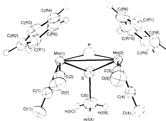
Fig. 3. A view of the molecule [\text{Mo}_2\text{Cp}_2(\mu\text{-H})(\mu\text{-SMe}(\text{CO})_4)] 4 showing 50% probability ellipsoids, except for Cp and methyl hydrogen atoms, which are represented by spheres of arbitrary radius.
