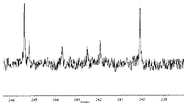
Fig. 2. ^{13}\text{C}\{^1\text{H}\} NMR spectrum of 7 in the CO region at 223 K.
