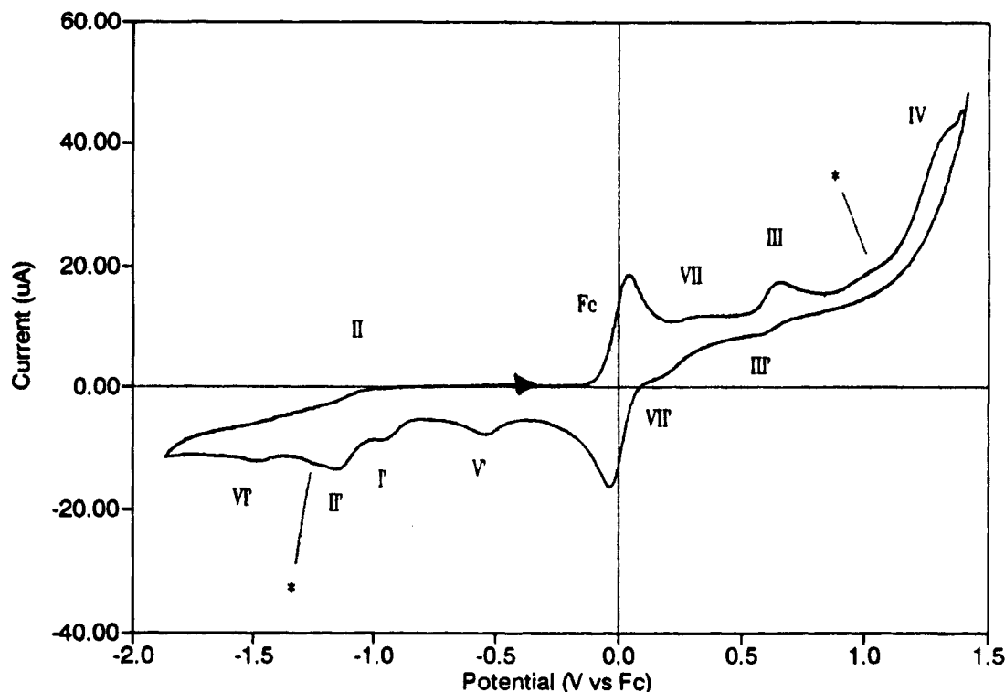
Figure 2. Oxidative cyclic voltammogram of [\text{Ni}(\eta^4\text{-P}_3\text{P}')\text{I}][\text{PF}_6] : 1 mM in 1 mM \text{Fc}/0.1 \text{ M NBu}_4\text{PF}_6/\text{MeCN} using a 0.86 mm radius platinum disk electrode at 0.25 V/s.
