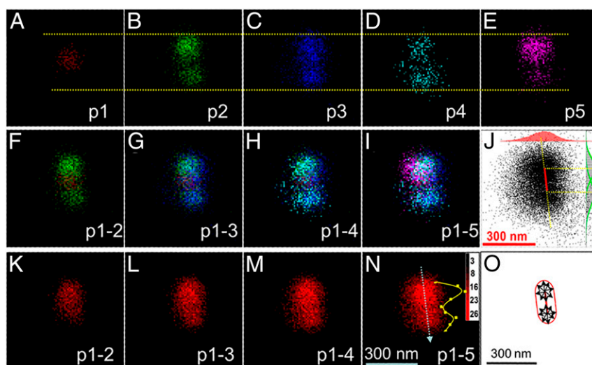
Fig. 2. Time-sequence single-molecule catalysis mapping on a single Sb-doped \text{TiO}_2 nanorod in 10 \times 10 \text{ nm}^2 bins. (A–E) The time sequence of 2D histograms of every 2,000 product molecules. Different colors indicate different portions of product molecules obtained in the time sequence [(A) p1: the first 2,000 product molecules; (B) p2: the second 2,000 product molecules; (C) p3: the third 2,000 product molecules; (D) p4: the fourth 2,000 product molecules; and (E) p5: the fifth 2,000 product molecules]. (F–I) The overlapping of different portions. (F) (p1-2) or (p1+p2); (G) (p1-3) or (p1+p2+p3); (H) (p1-4); (I) (p1-5). (J) Positions of product molecules detected on the nanorod in I. (Insets) Histogram distribution in both X (up) and Y (right) directions. (K–N) The 2D histograms of different numbers of product molecules obtained on the rod at different time: (K) The first 4,000 product molecules; (L) The first 6,000 product molecules; (M) The first 8,000 product molecules; (N) All of the (around 10,000) product molecules; (Inset) Intensity distribution along the long-axis direction. (O) Scheme to show the limited spatial-resolution and molecule diffusion-induced smearing of the outline of the nanorod.
