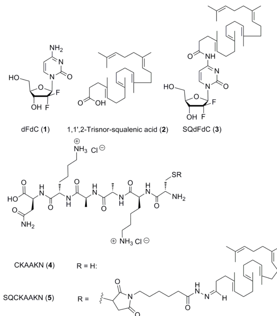
Fig. 1. Squalenoyl derivatives.
