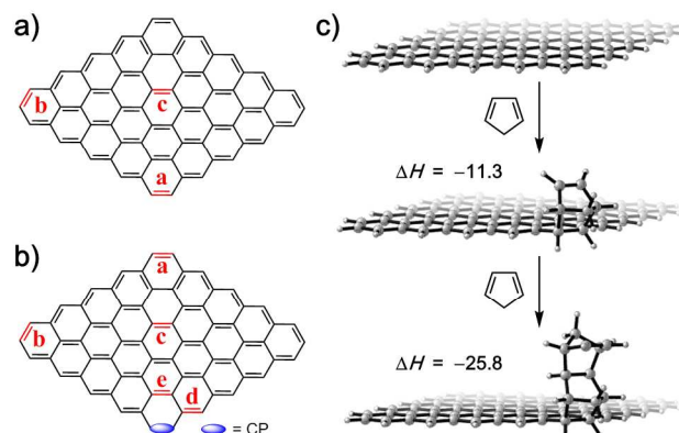
Figure 5. a) The 5x5 graphene model with the representative addition sites in red. b) DA reaction sites of the second CP on graphene-CP cycloadduct. c) Structures of graphene, graphene-CP cycloadduct, and the following CP dimerization product, reaction enthalpies in kcal/mol.
