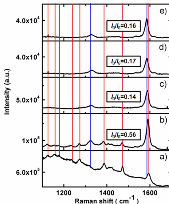
Figure 3. a) Raman spectrum of 1 on a SiO 2 surface. b) Raman spectrum from a map with force accelerated printing of 1 (Fig. 2b) taken at a position with increased D-band intensity ( I_D ) compared to unreacted SLG also has peaks corresponding to 1 . c) Raman spectrum from the map of the same printed surface taken at a position without increased I_D . d) Raman spectrum of control experiment where PEG and force were applied to the SLG surface without 1 , taken at a point where the tips were pushed into the SLG surface. e) Raman spectrum of pure SLG. Red lines mark peaks of 1 (11124, 1157, 1178, 1272, 1387, 1594 \text{cm}^{-1} ). Blue lines mark SLG peaks (1324, 1584 \text{cm}^{-1} ).
