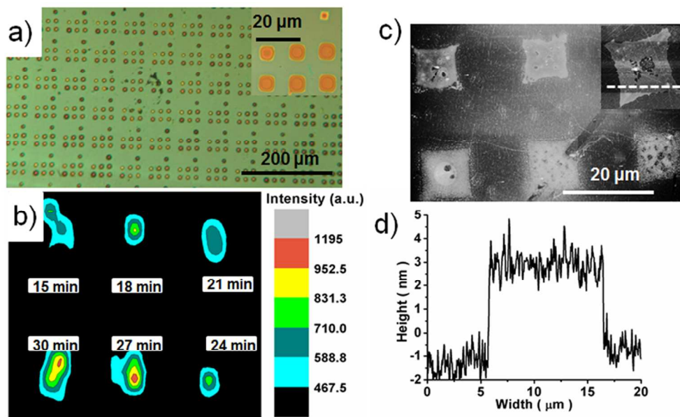
Figure 2 a) Light microscopy image (10x magnification) of 2 x 3 dot arrays of a mixture containing 1 and PEG, with varying dwell times (30, 27, 24, 21, 18, 15 min), that were patterned by each pen in the tip array. Scale bar is 200 μm. Inset is a magnified image of one array. Scale bar is 20 μm. b) Raman mapping image (1324 cm -1 , D band) of 2 x 3 dot arrays of 1 covalently immobilized onto the SLG. Scale bar is 20 μm. c) AFM image of a single feature printed onto the SLG. d) Height profile of a single feature of 1 patterned onto SLG. 85x50mm (300 x 300 DPI)
