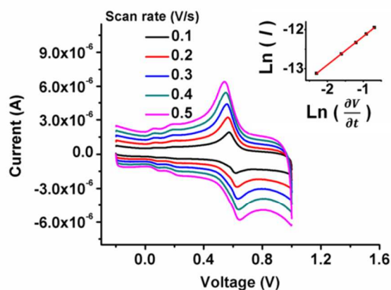
Figure 4. Cyclic voltammetry (CV) of 2 on SLG using a Pt counter electrode and Ag/AgCl reference electrode in 0.1 M HClO 4 electrolyte. The inset shows the relationship between \ln(\text{scan rate}) and \ln(\text{current}) .
