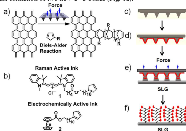
Figure 1. a) DA oligomerization reaction between functionalized CP and a single layer graphene (SLG) surface. b) Cy3-containing Raman active 1 and ferrocene-containing electrochemically active 2 ink molecules used to confirm force-accelerated patterning. c) An elastomeric tip-array. d) The tip-array coated with an ink mixture (red) consisting of a CP and poly(ethylene glycol) (PEG). e) The inked tip array is pushed into the SLG surface. f) Following rinsing of the surface to remove the PEG and excess CP, only the covalently immobilized molecules remain on the surface.
