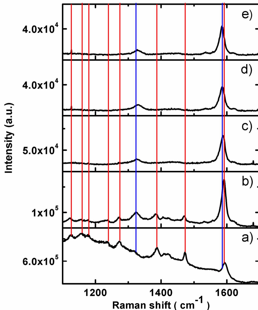
Figure 3 a) Raman spectrum of 1 on a \text{SiO}_2 surface. b) Raman spectrum from a map with force accelerated printing of 1 (Fig. 2b) taken at a position with increased D-band intensity (ID) compared to unreacted SLG also has peaks corresponding to 1. c) Raman spectrum from the map of the same printed surface taken at a position without increased ID. d) Raman spectrum of control experiment where PEG and force were applied to the SLG surface without 1, taken at a point where the tips were pushed into the SLG surface. e) Raman spectrum of pure SLG. Red lines mark peaks of 1 (11124, 1157, 1178, 1272, 1387, 1594 \text{cm}^{-1} ). Blue lines mark SLG peaks (1324, 1584 \text{cm}^{-1} ). 279x371mm (150 x 150 DPI)
