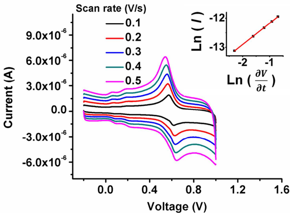
Figure 4 Cyclic voltammetry (CV) of 2 on SLG using a Pt counter electrode and Ag/AgCl reference electrode in 0.1 M HClO 4 electrolyte. The inset shows the relationship between \ln(\text{scan rate}) and \ln(\text{current}) . 85x64mm (300 x 300 DPI)
