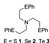
Scheme 1. Systems Used in This Study
