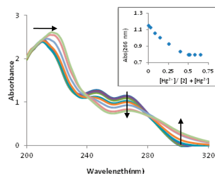
Figure 1. Absorption spectra of 2 (100 \mu\text{M} ) in 80:20 (v/v) \text{CH}_3\text{CN} – \text{H}_2\text{O} and changes observed upon the addition of a \text{Hg}(\text{NO}_3)_2 salt solution (0–100 \mu\text{M} ) in \text{H}_2\text{O} . Inset: Job's plot showing minima at 0.50, indicating 1:1 binding between 2 and \text{Hg}^{2+} .
